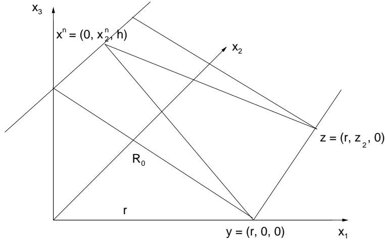
Figure 3: This shows the geometry for computation of the azimuthal resolution.
