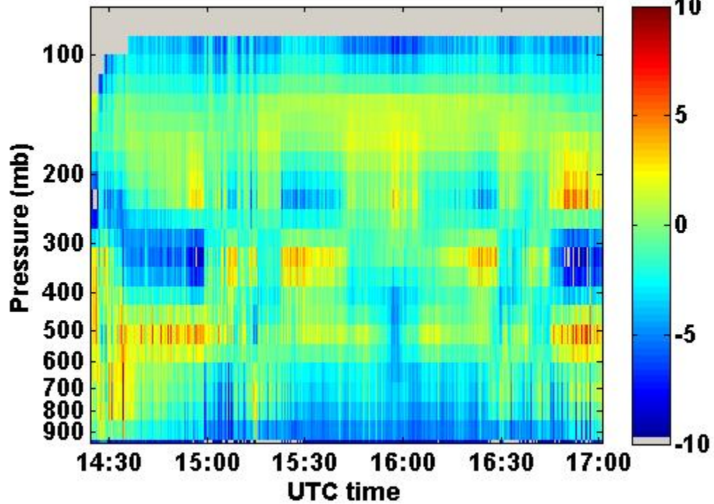
HAMSR-MERRA T(z) °C 17-Sep-2013 13:08:37 to 17-Sep-2013 18:01:18
