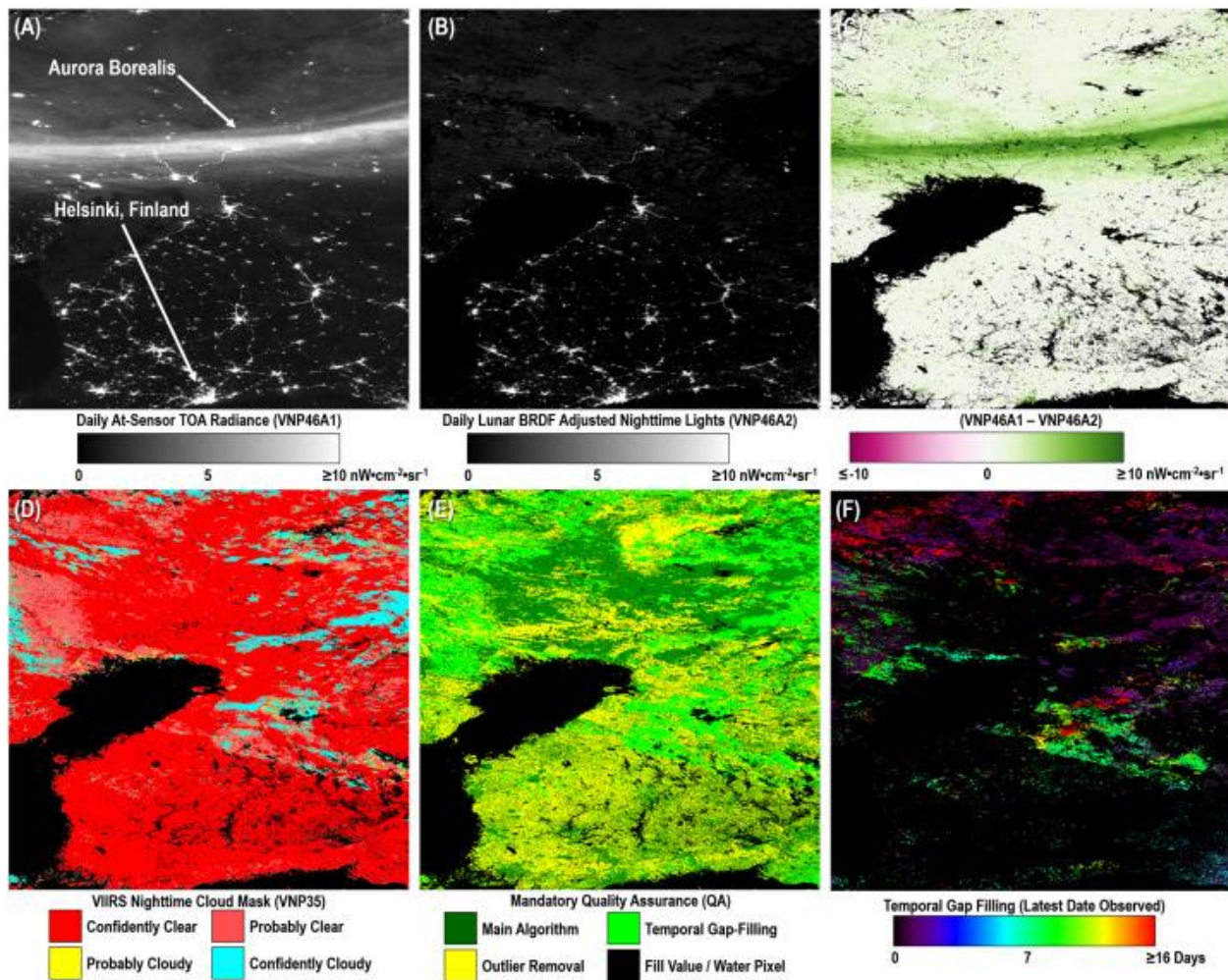
Figure 5 VNP46 product suite components for a 10° × 10° Level 3 tile over Sweden and Finland (h20v02; DOY 2013-080). The half-moon-illuminated and 30% cloud-contaminated scene is shown to capture extraneous light emissions north of the Gulf of Bothnia caused by the Aurora Borealis.
