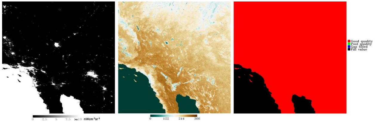
Figure 6 VNP46A3 monthly (upper) and VNP46A4 yearly (bottom) NTL composite (left), the associated number of observations for the composite (middle) and quality (right) for a 10^\circ \times 10^\circ Level 3 tile h06v05 in 2016.
