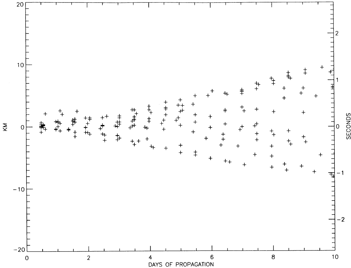
Fig. 11. SGP4 along-track propagation errors for LANDSAT-5: 0–10 days.
