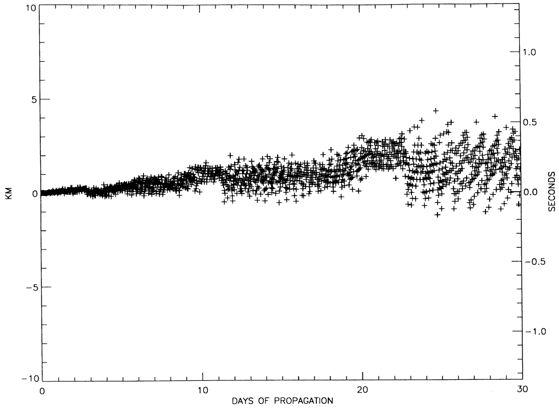
Fig. 14. Along-track propagation differences between SGP4 and DCF/SGP4.
