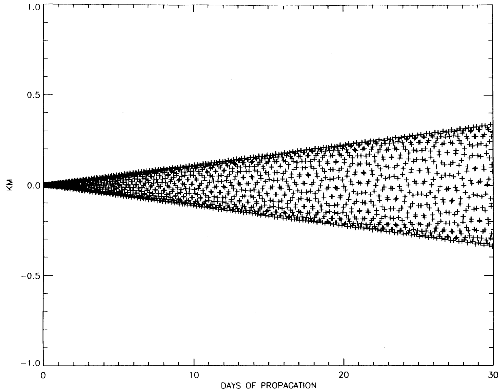
Fig. 17. Cross-track propagation differences between DCF/Brouwer and NOAA/Brouwer.
