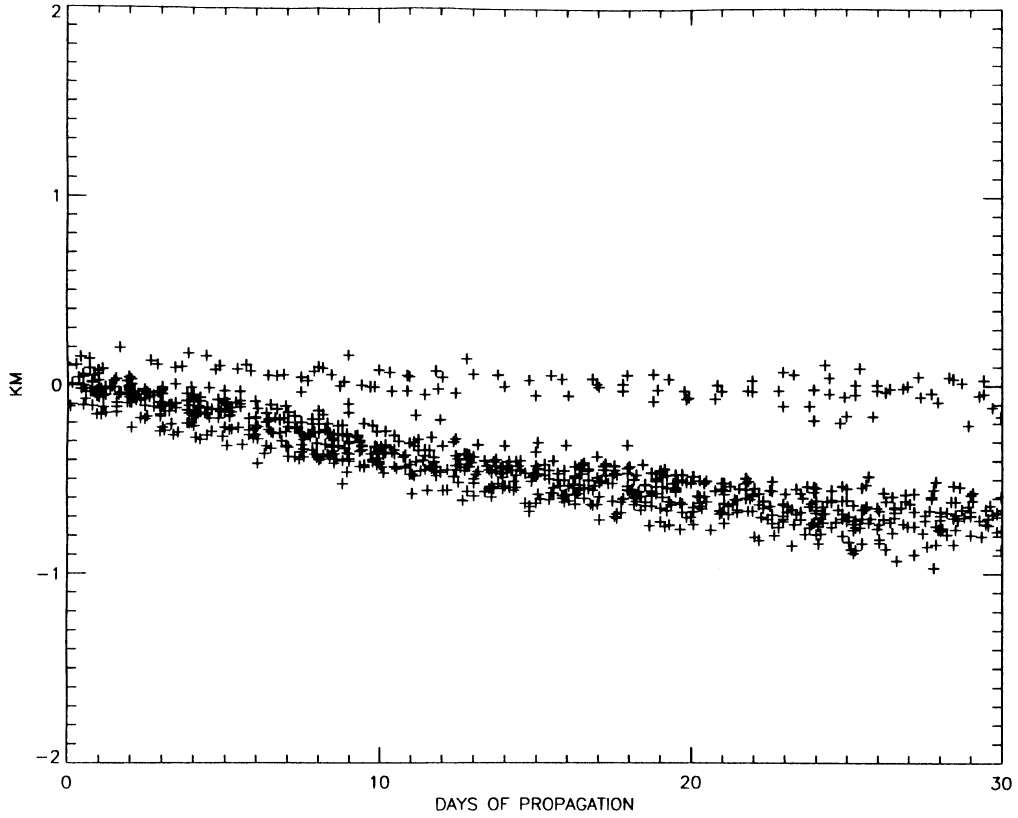
Fig. 10. DCF/SGP4 radial propagation errors for NOAA-12: 0–30 days.
