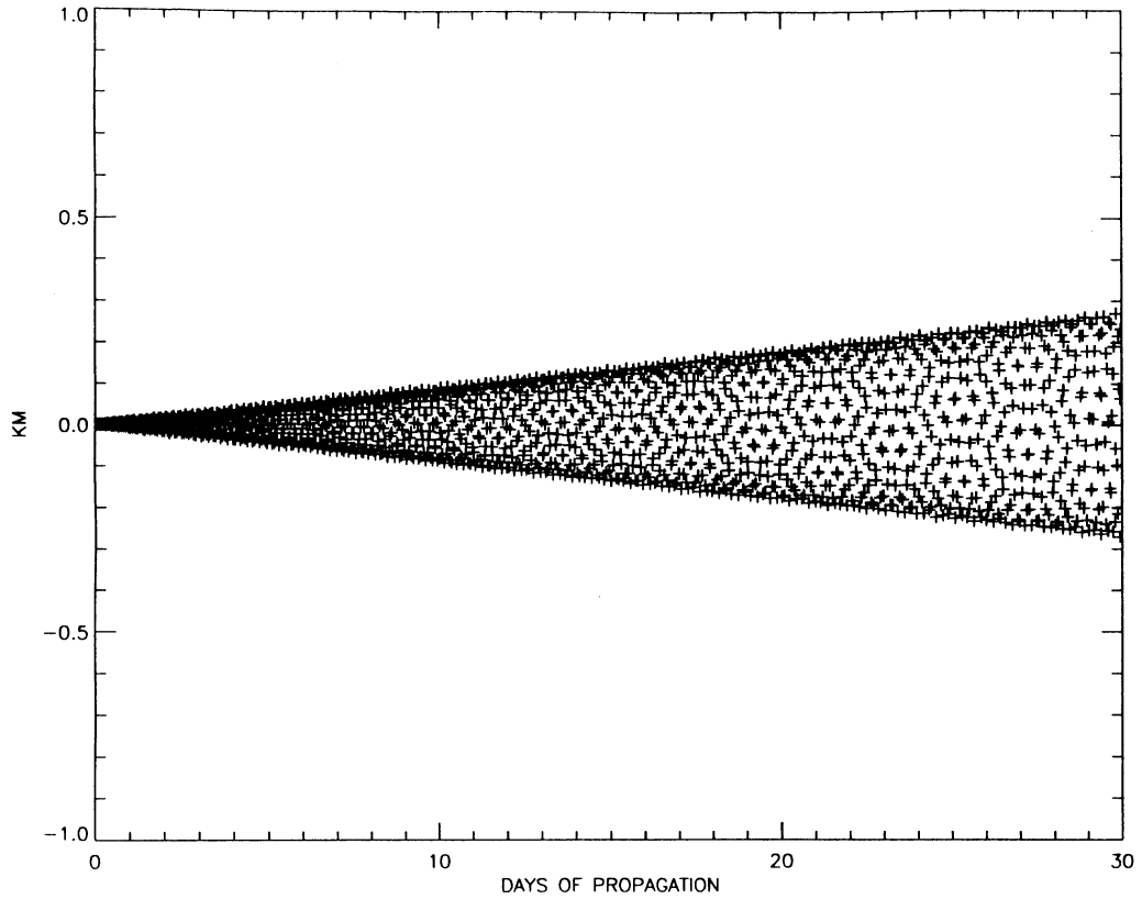
Fig. 15. Cross-track propagation differences between SGP4 and DCF/SGP4.
