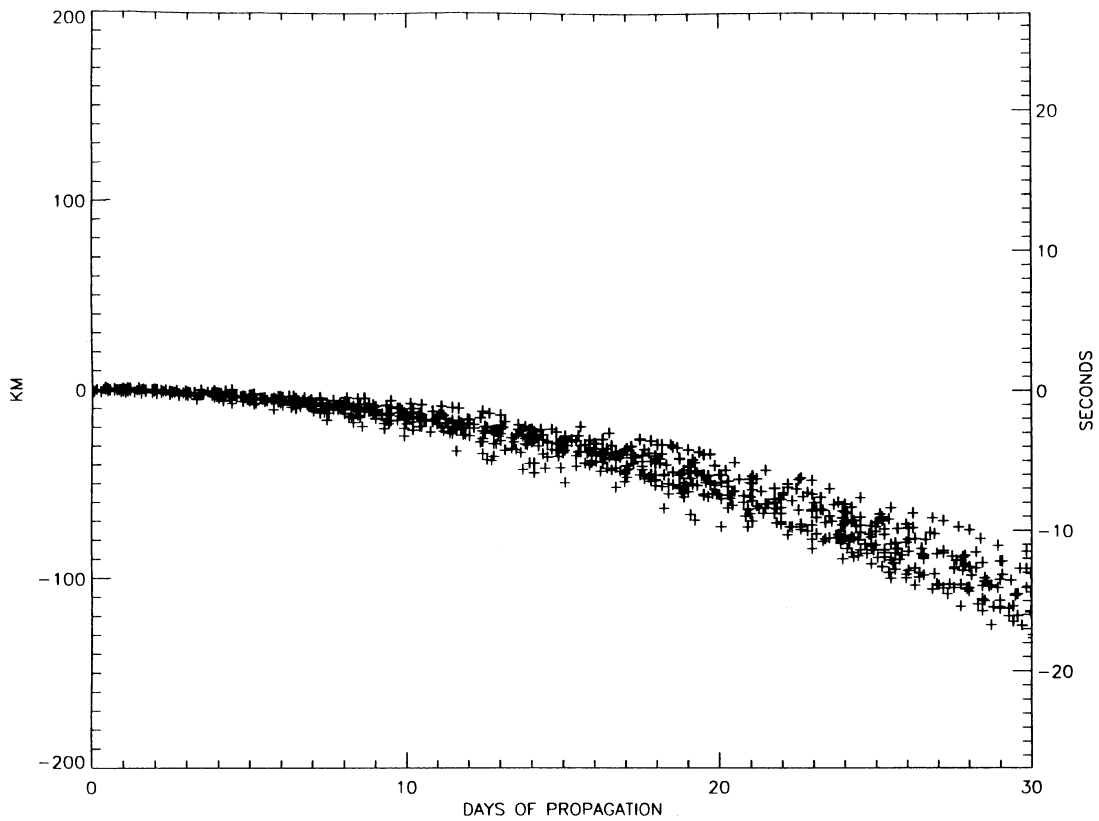
Fig. 8. NOAA/Brouwer along-track propagation errors for NOAA-12: 0–30 days.
