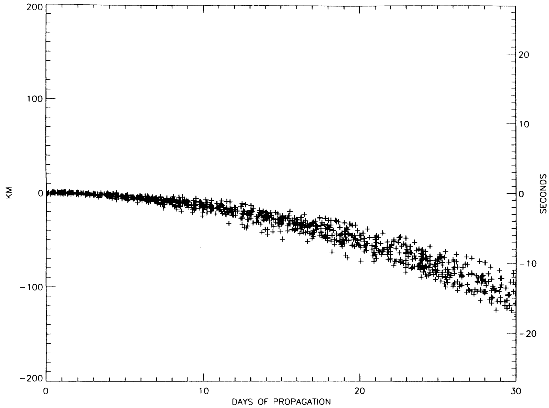
Fig. 6. DCF/Brouwer along-track propagation errors for NOAA-12: 0–30 days.
