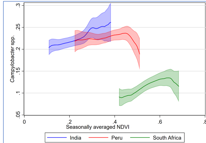
Relationship between NDVI at Campylobacter infection rates at three study sites.
