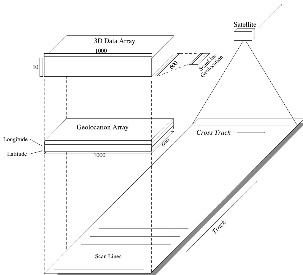
Figure 6.1-3 Conceptual View of Example Swath, with 3D Time/Geolocation Array, and Geolocation Table.
