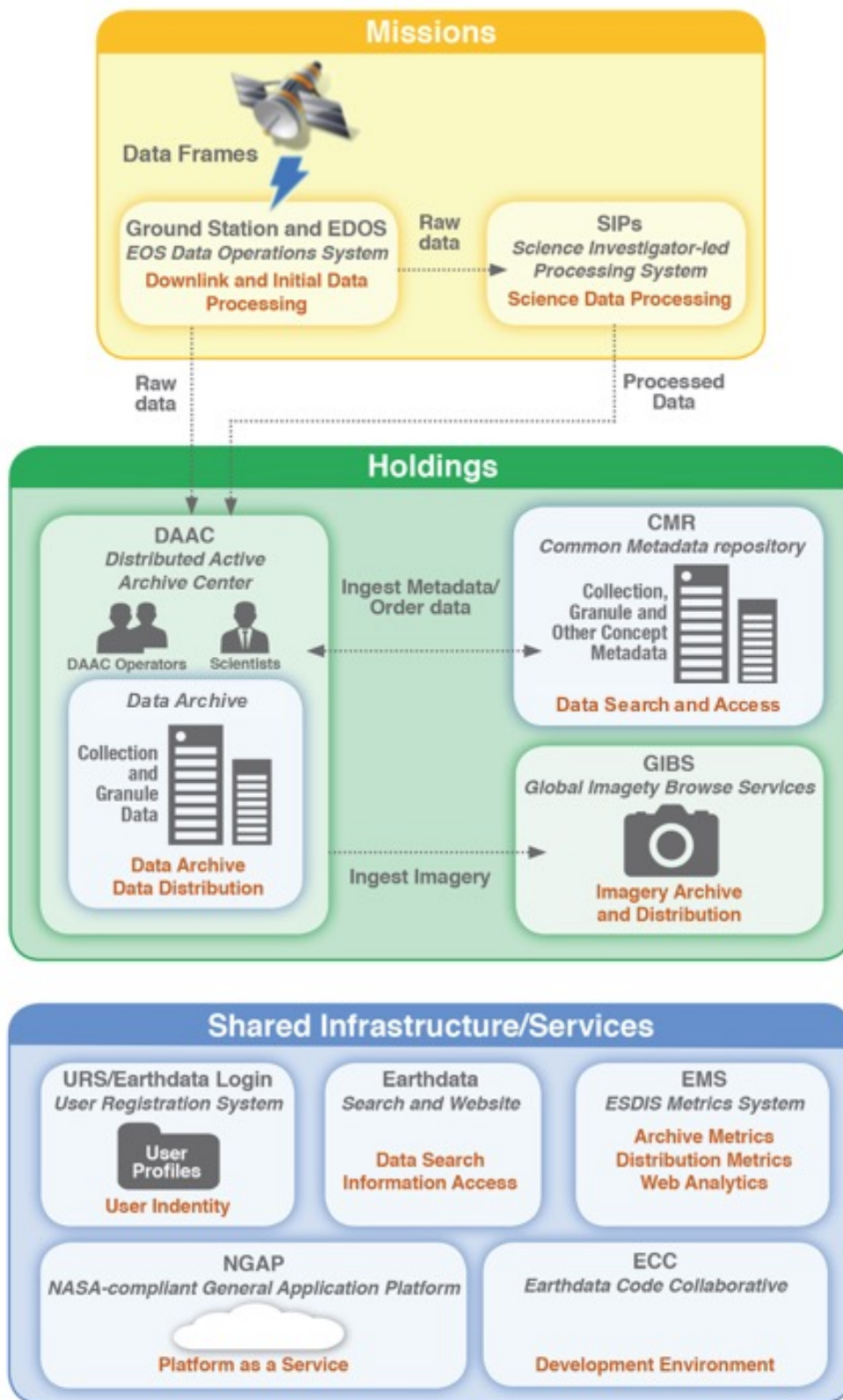
Figure 7: EOSDIS overview and common services
