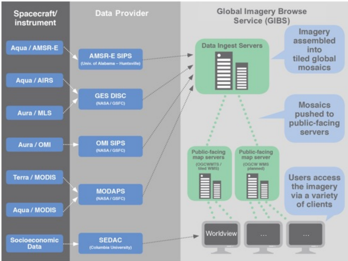
Figure 12: GIBS imagery comes from a variety of data collections and is available through standard APIs
