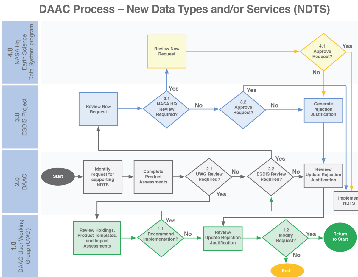
Figure 19. DAAC process for adding new data types or services to the collection.
