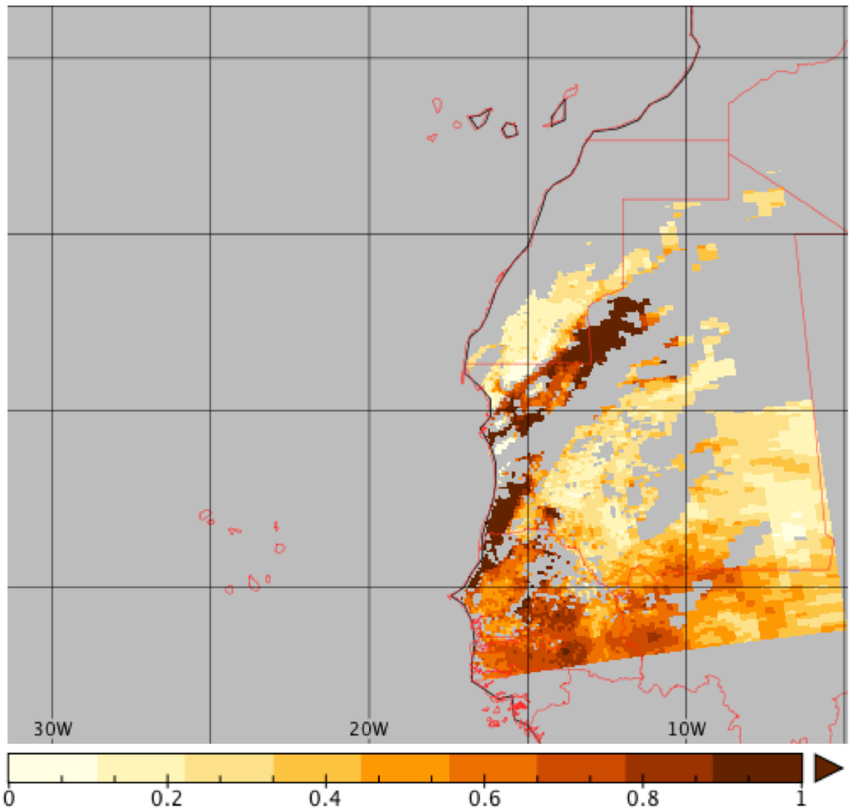
Figure 14: Aerosol Optical Depth retrieval from MODIS on Aqua 5 , 28 March 2008.
