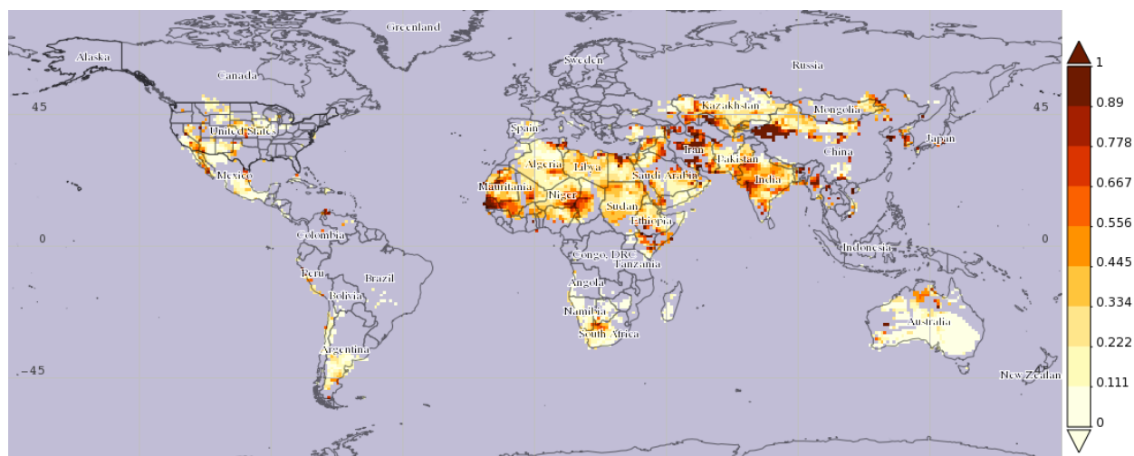
Figure 15: Level 3 gridded Aerosol Optical Depth (Deep Blue Algorithm) for MODIS on Aqua satellite, 28 March 2008.
