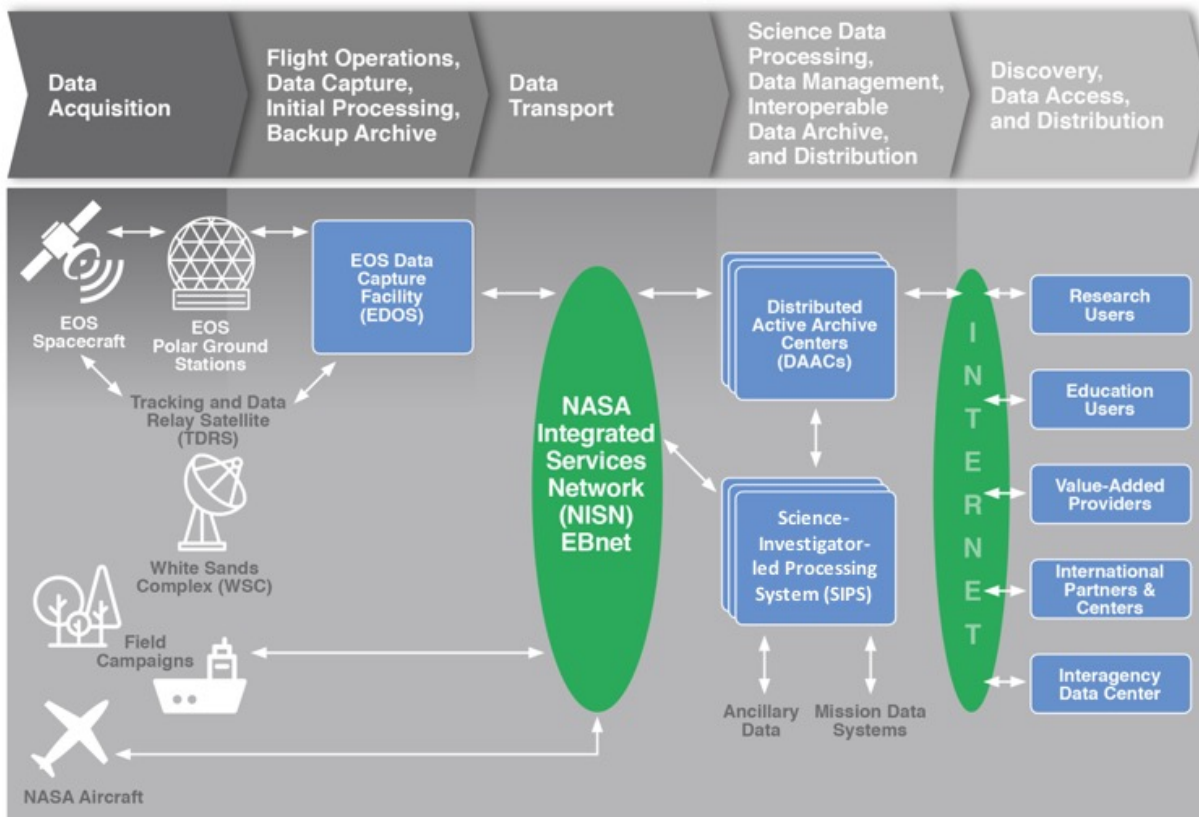
Figure 1: EOSDIS data lifecycle from acquisition to distribution
