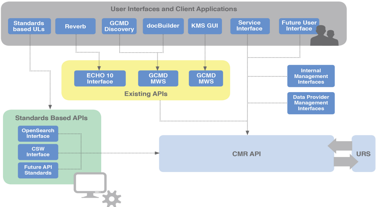
Figure 8: High-level overview of key CMR interfaces
