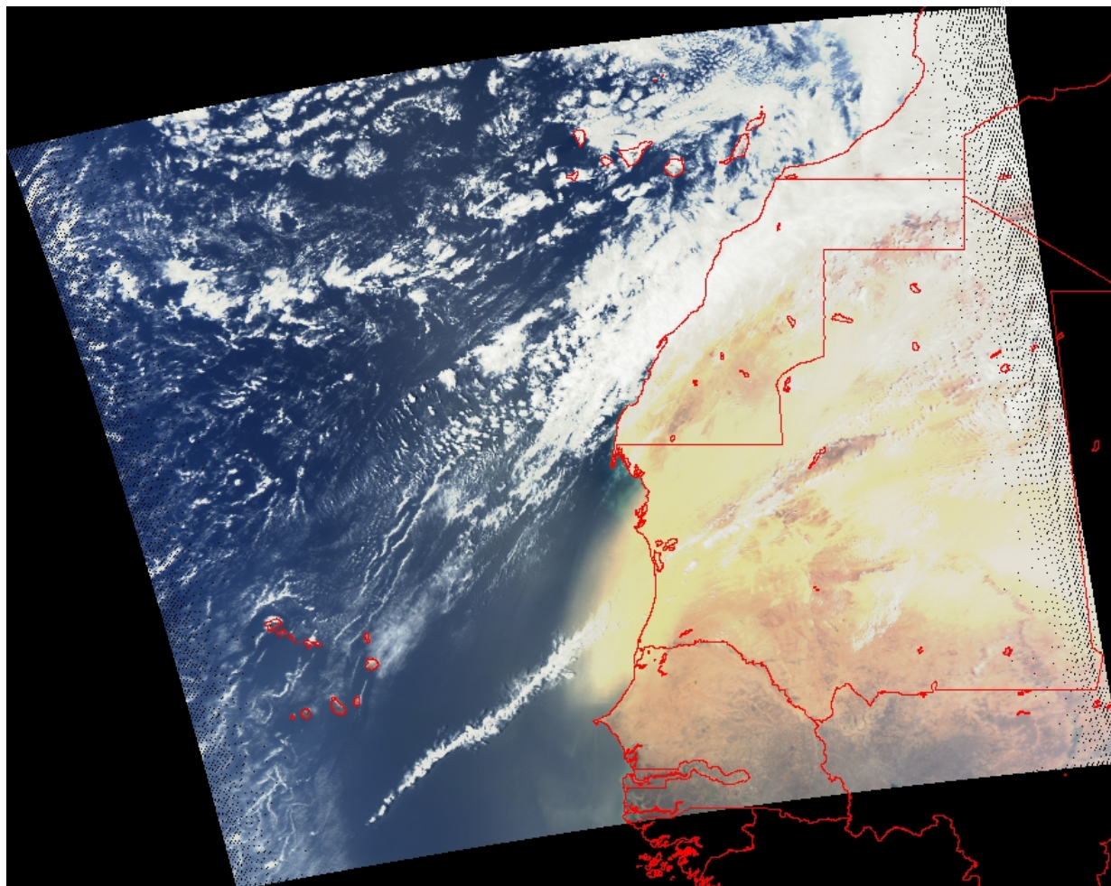
Figure 14: Level 1B Calibrated Radiance from MODIS on Aqua, 28 March 2008. The image approximates true color, using MODIS Band 1 for Red, Band 4 for Green, and Band 3 for Blue 3 .
