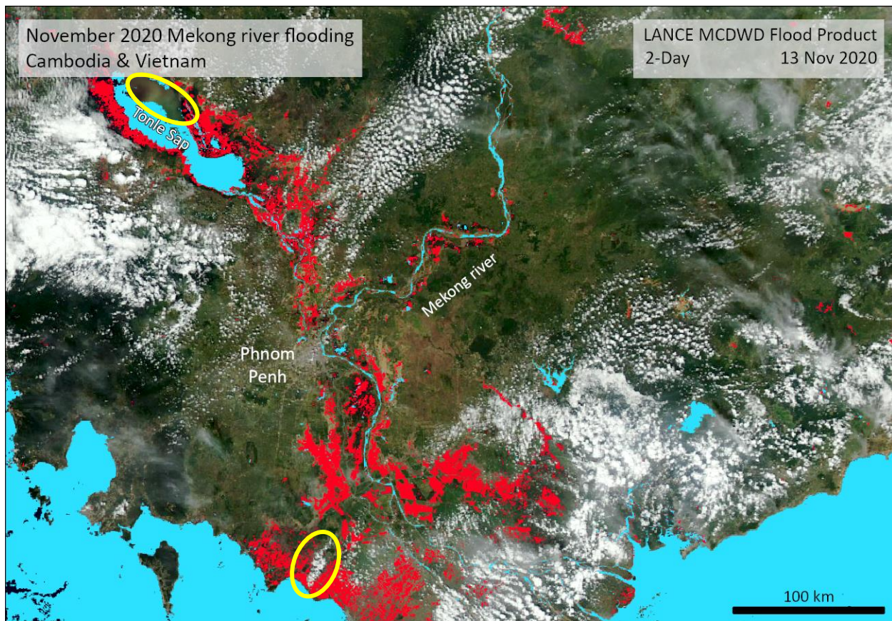
Figure 6: Example: The 2-Day flood product showing extensive flooding in the lower Mekong region of Cambodia and Vietnam, overlaid on MODIS-Aqua imagery from 13 Nov 2020. Upper yellow polygon shows portion of Tonle Sap lake not being detected in this composite, even though this particular Aqua image appears relatively clear; that area reappears in the 1-Day composite due to water detections from this Aqua image. Lower polygon shows an area where cloud in this Aqua image is obscuring likely flood detection.
