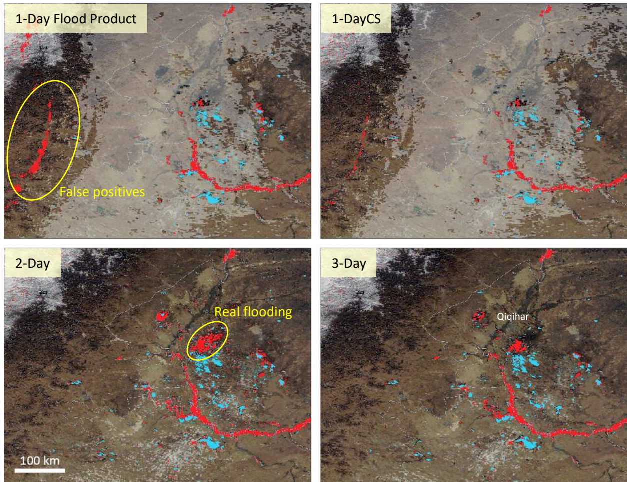
Figure 12: Demonstration of the difference between the four products: 1-Day, 1-Day CS (with Cloud Shadow screening), 2-Day, and 3-Day, during flooding of Songhua river, NE China, 26 Oct 2020. Yellow outline in 1-Day panel shows area of cloud-shadow false-positive, which is substantially ameliorated in the 1-Day CS product (but not entirely), and is completely removed from the 2 and 3-Day products. Yellow outline in 2-Day panel shows an area of flooding that is only here captured in the 2-Day product; the 1-Day products had some cloud over this in both Terra and Aqua, and the 3-Day suggests there were not sufficient water observations (3) in the two previous days, for this to be captured. It is possible the water was not fully present on the two previous days if this is a rapidly evolving event, or that there was cloud obscuration; a review of the contributing MODIS imagery would be needed to make a clear determination.
